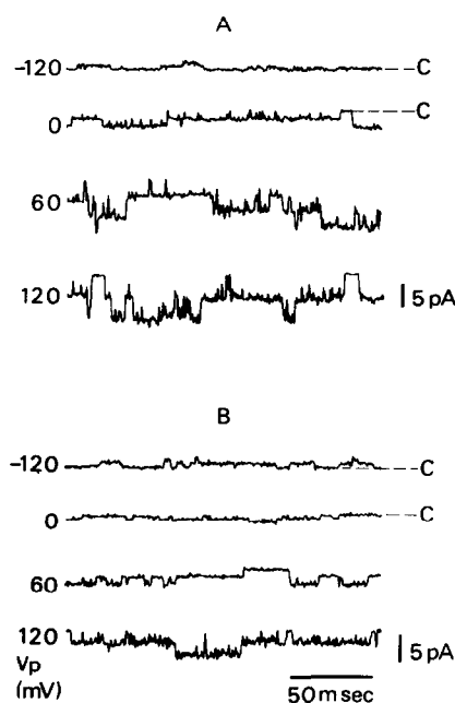
Fig. 2. Conductance and ion selectivity of the ATP-induced single-channel currents. (A, B) Expanded current records corresponded to part c of Fig. 1A with the symmetrical 145 mM KCl (A) or 36 mM KCl (B) pipette solution at different V_p (indicated to the left). (C) I-V relations from (A) (open circles) and (B) (open squares). Data points are mean \pm SD. Number of patches used to determine each point is shown in parentheses.
